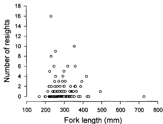
Fig. 4 Number of resights of individually tagged snapper ( Pagrus auratus ) plotted against fork length at tagging (excludes tagged fish not positively identified).
